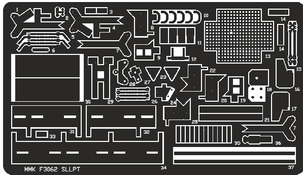
PHOTO-ETCHED PARTS
