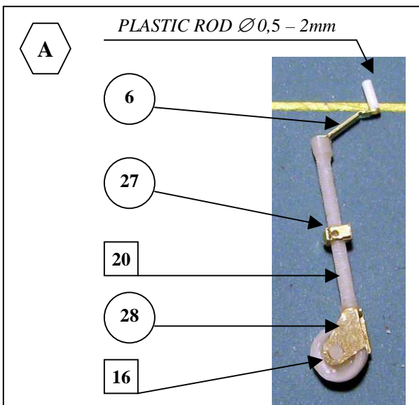
PHOTO-ETCHED PARTS
